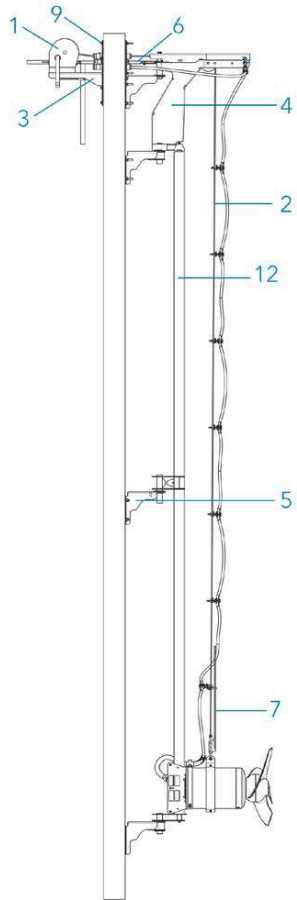
BIS-1 support system side view
